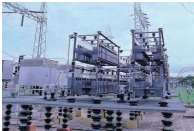
India's first Fixed Series compensation scheme at Ballabhgarh (Haryana), India
