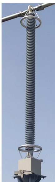
400kV Optical Current Transformer (CT)
